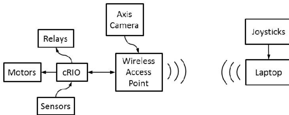
FIGURE 3.1 Schematic diagram of an FRC robot control system.
