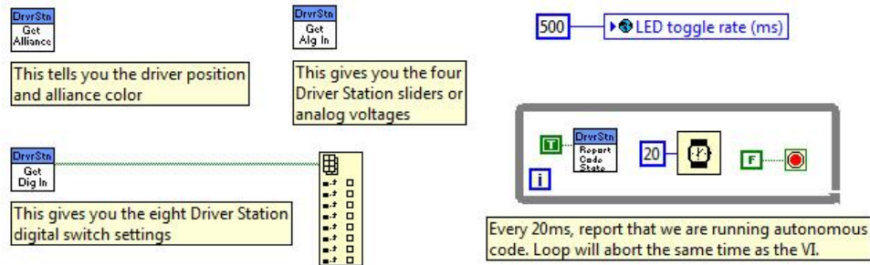
FIGURE 4.14 The “standard” bits of Autonomous Independent.vi.
