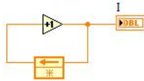
FIGURE 1.18 And yet another implementation of I = I + 1 .
