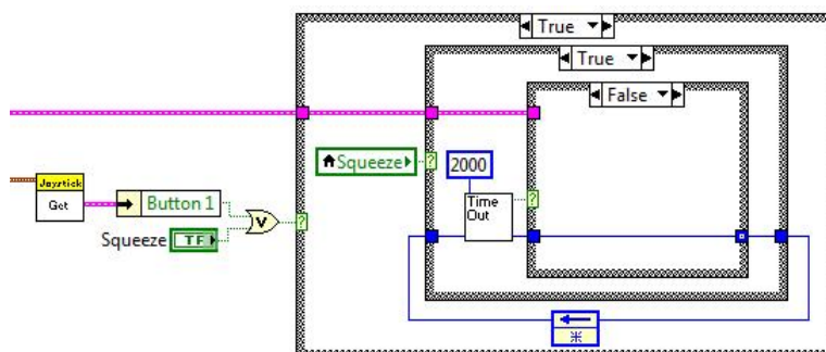
FIGURE 4.9 The code that runs after the button is pressed but before 2 seconds has elapsed.
