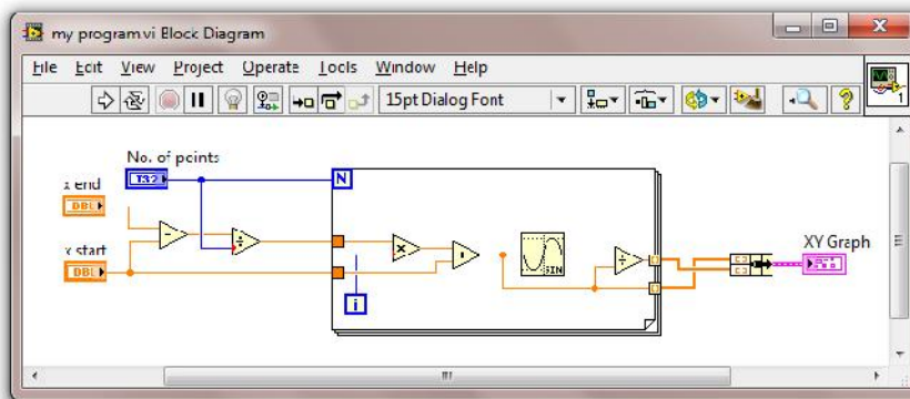
FIGURE 1.4 The block diagram of the program in Fig. 1.3.
