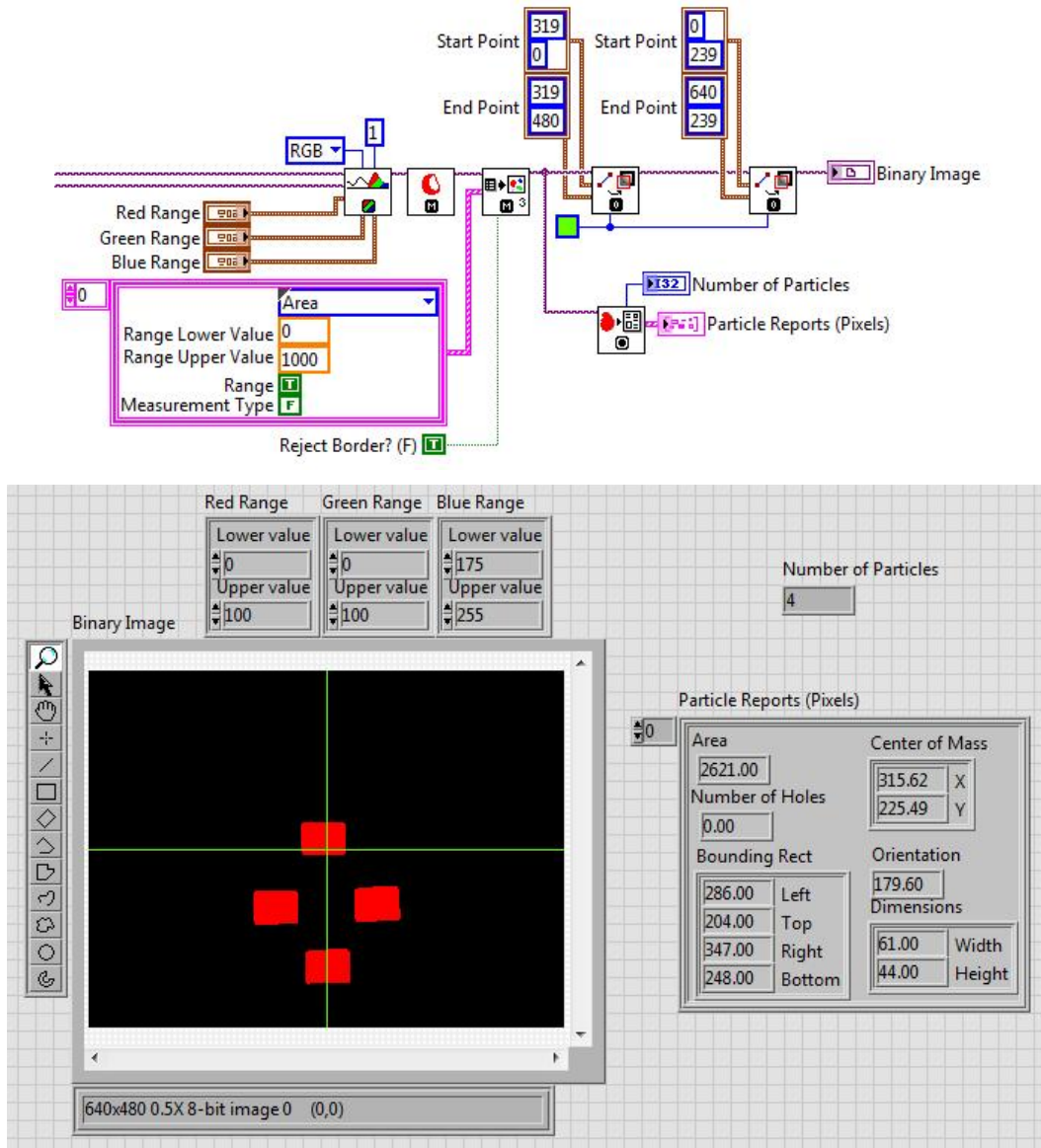
FIGURE 7.10 A complete BLOB finding program.
