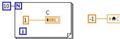
FIGURE 1.19 And yet another implementation of I = I + 1 .
