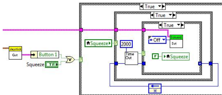
FIGURE 4.10 The end of the delay.
