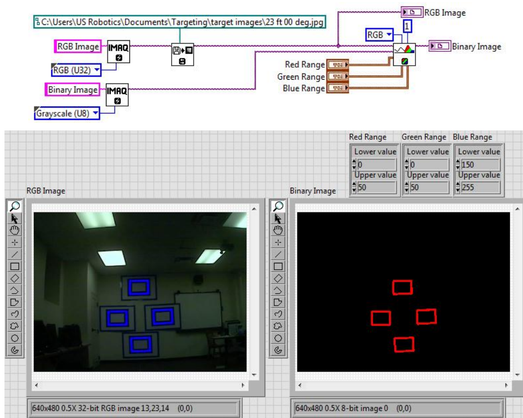
FIGURE 7.9 The first stage in BLOB finding: identifying the target pixels.
